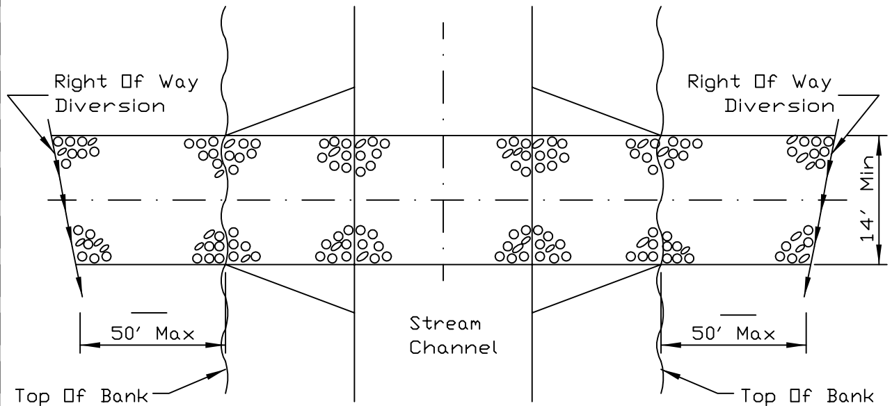
PLAN VIEW
