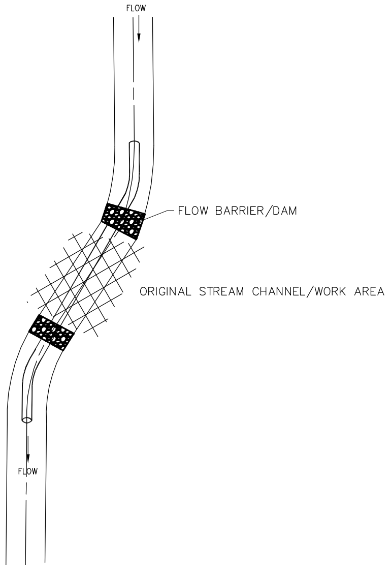
TYPICAL PIPE DIVERSION PLAN
