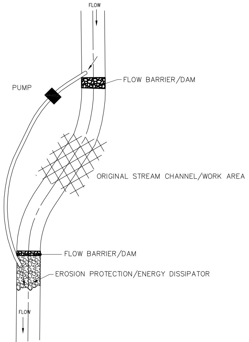
TYPICAL PUMPED DIVERSION PLAN
